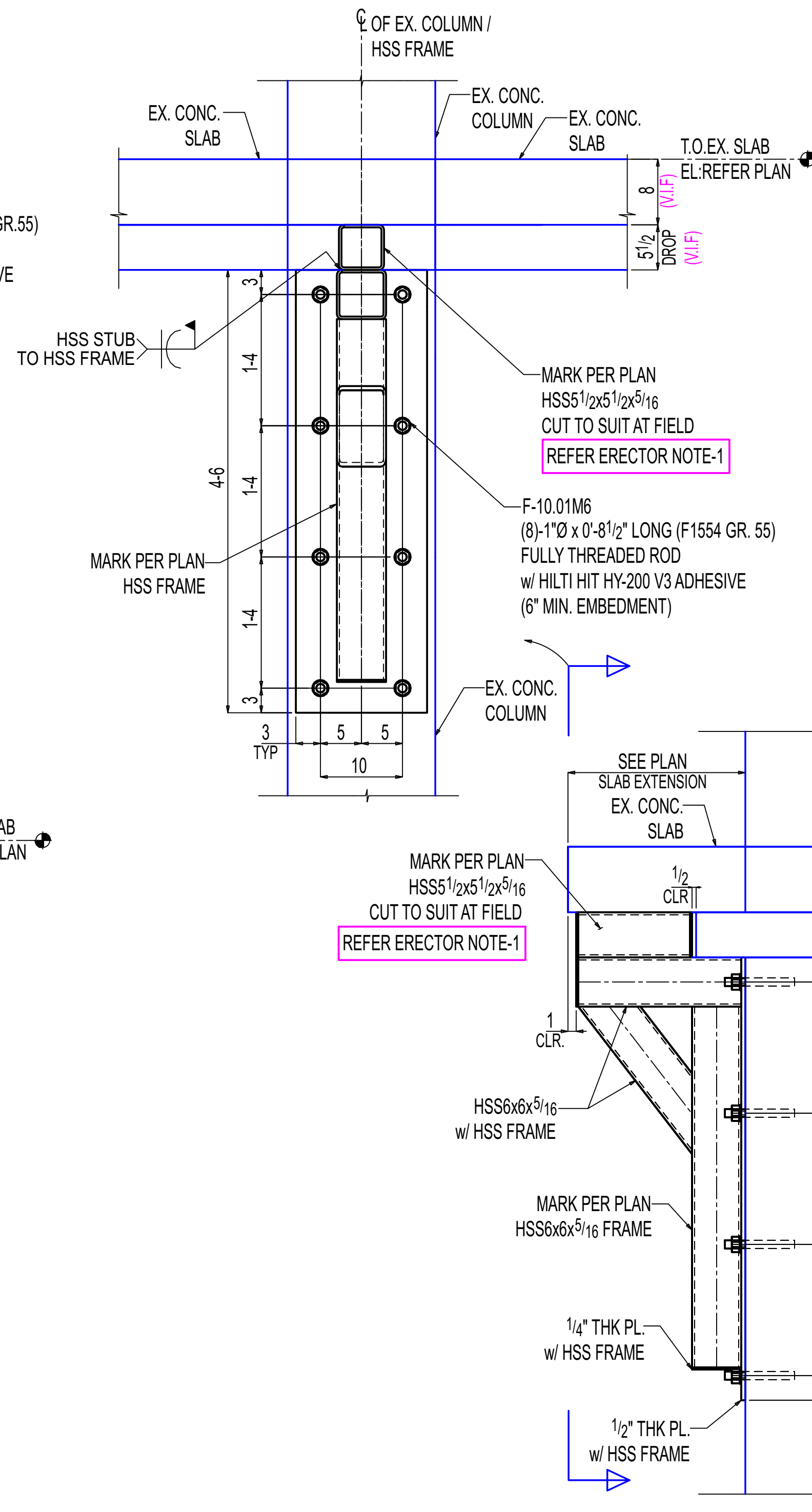
B-B (NEW SLAB EXTENSION SUPPORT 1'-6" TO 3'-1") E-10.00 (REF:3 & 4/S307) OTHERS NOT SHOWN FOR CLARITY
